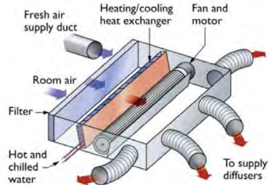
Figure 2. Basic configuration of a horizontal fan coil unit (BSRIA, 2013).
