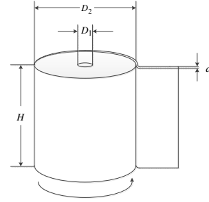
Fig. 14. The winding process of electrolytic capacitor.
