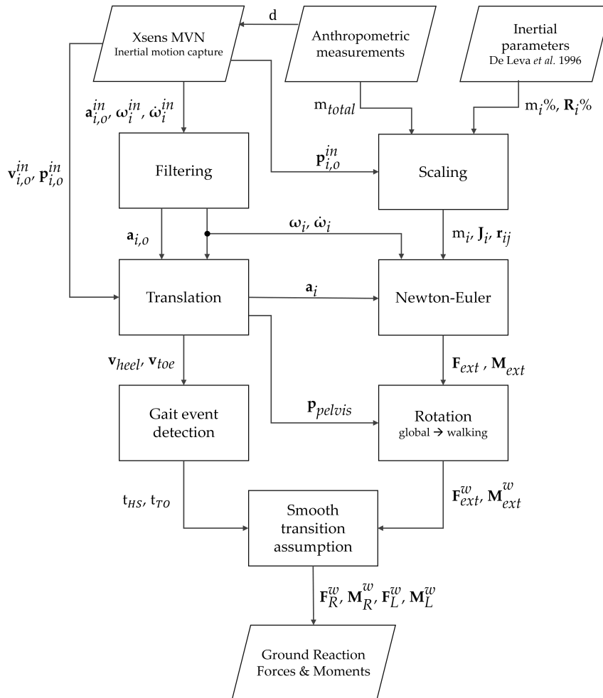
Figure 5. Block diagram of the algorithm used to estimate the GRF&M from anthropometry and inertial motion capture. \mathbf{p} = position, \mathbf{v} = velocity, \mathbf{a} = acceleration, \omega = angular velocity, \dot{\omega} = angular acceleration, \mathbf{F} = force, \mathbf{M} = moment, t = time, d = anthropometric dimensions, m = mass, \mathbf{R} = radius of gyration, \mathbf{J} = inertia tensor. Superscript “in” indicates quantities derived directly from the IMC system, and w denotes quantities expressed in the coordinate system defined by the walking direction. Subscript i indicates a variable of the i -th segment. Additional subscript o denotes that a linear variable is expressed in the origin of the segment, whereas no additional subscript denotes that it is expressed in the center of mass of the segment. Subscript ext = external, R = right, L = left.
