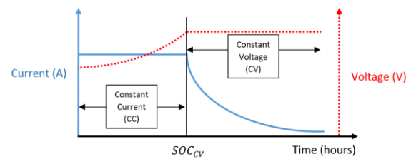
Fig. 4. CC-CV charging method of the BESS.
