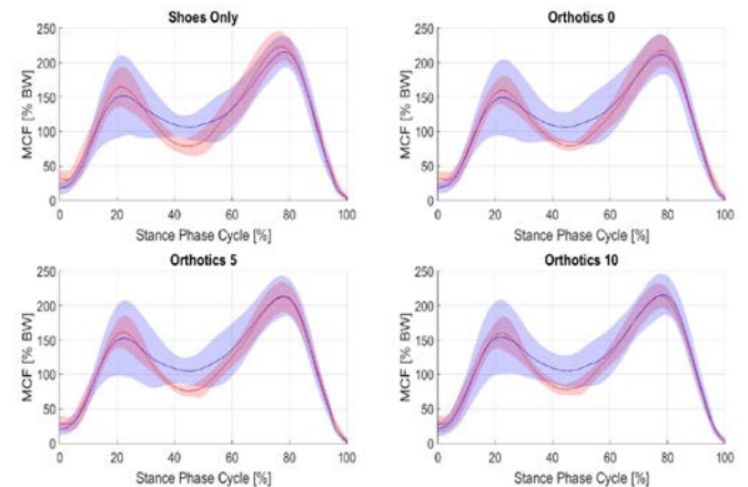
Figure 1: Knee Medial Compressive Force (MCF) for control (red) and medial KOA with varus malalignment (blue). Shaded areas indicates \pm 1 standard deviation.
