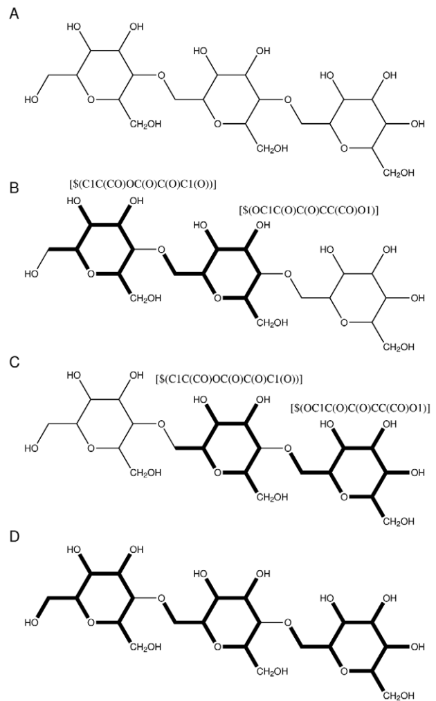
Figure 5. Sugar Fragmentation Example. An example of how fragmentation is carried using SMARTS patterns on a polysaccharide molecule in FragIt. Illustration a) is the polysaccharide molecule of interest, in this case an D-galactopyranose trimer. b) and c) shows examples of fragmentation using the polysaccharide fragmentation pattern in this work. Finally, d) shows the final fragmentation of 3 fragments.
