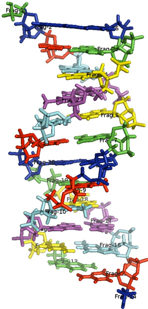
Figure 6. Fragmentation of DNA using FragIt. We use a six color coloring scheme resulting in different fragments may have the same color.
