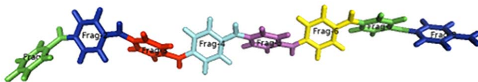
Figure 7. Fragmentation of Leucoemeraldine (a Polyaniline) using FragIt. This particular example uses no fragmentation patterns but rather explicitly defined points of fragmentation by the end user.
