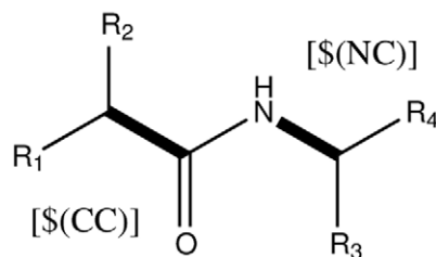
Figure 2. Pattern matching on a peptide bond using SMARTS. doi:10.1371/journal.pone.0044480.g002
