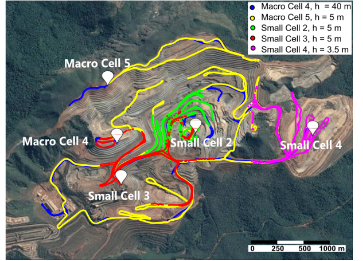
Figure 2. Measurement routes and transmitter positions in Mine 2. The height above ground level, h , is also displayed in the legend.
