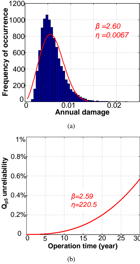
Fig. 6. Monte Carlo analysis considering all parameter variations from the stress evaluation and lifetime model for the most stressed MOSFET Q_{ps} . (a) Annual damage distribution; (b) Accumulated percentage of failure (i.e. unreliability) along with the operation time.
