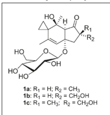
Structures of norsesquiterpenoid glycosides: 1a: Ptaquiloside; 1b: Ptsculentoside; 1c: Caudatoside. (Modified from Fletcher, M.T., et al. 2011)
