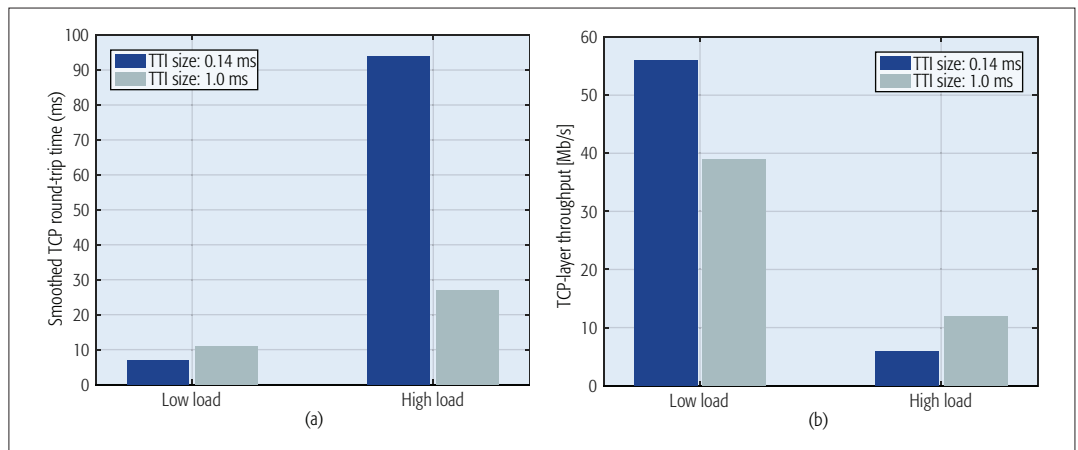
Figure 4. Performance of eMBB with different TTI sizes: a) smoothed median TCP packet round trip time; b) median TCP-layer end-user throughput.
