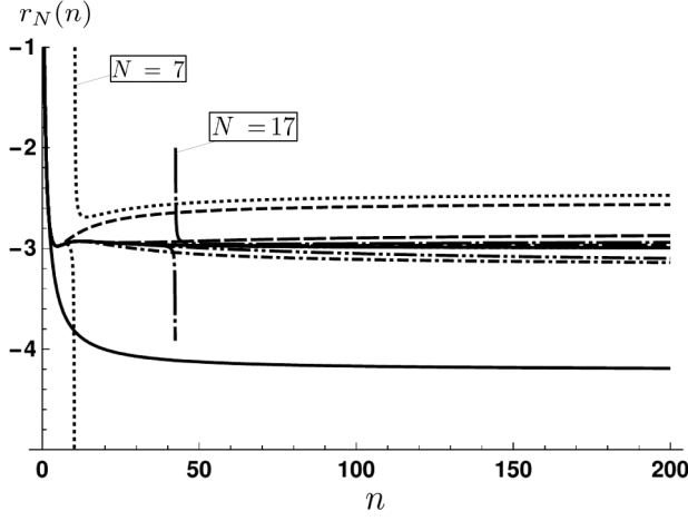
FIG. 3. Hypergeometric ansatz for the quartic anharmonic oscillator. We plot all the rational functions r_N(n) for N \leq 25 as a function of n ; these functions approximate the ratio between consecutive coefficients and are used to parametrize hypergeometric approximants in the Borel plane and Meijer- G approximants in the complex- g plane. While we observe good convergence with increased N we note that for N = 7 and N = 17 , the rational functions have poles for positive n , which spoil those two approximants.
