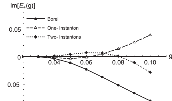
FIG. 11. Nonperturbative ambiguity as a function of coupling strength calculated for the quantum mechanical double-well problem. One- and two-instanton contributions reduce the size of the ambiguity but do not entirely cancel it in the interval 0.03 < g < 0.1 .
