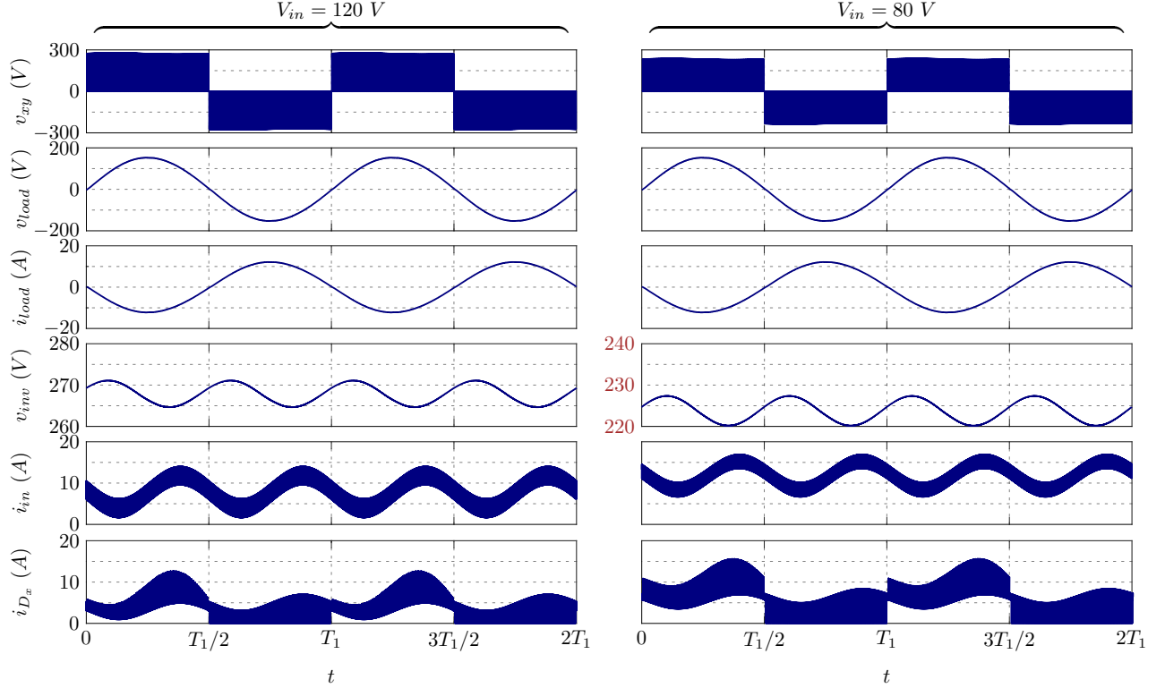
Fig. 6. Simulation results of the 1-kVA single-phase SSI using leading-edge sawtooth carrier for two fundamental cycles, considering V_{in} = 120 V and 80 V. From top to bottom: output voltage ( v_{xy} ), load voltage ( v_{load} ), load current ( i_{load} ), dc-link voltage ( v_{inv} ), inductor current ( i_{in} ), and diode D_x current ( i_{D_x} ).
