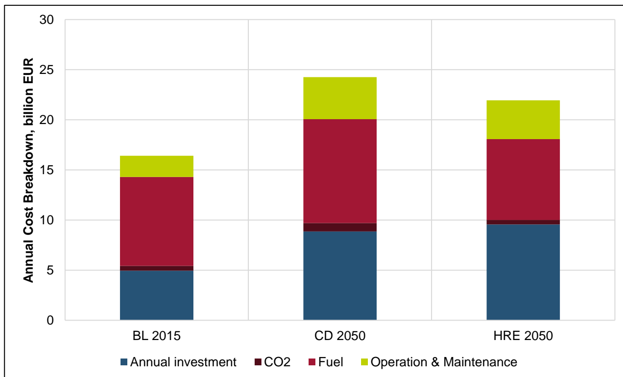
Figure 12. Annual socio-economic costs for the heating, cooling, electricity, industry, and transport sector for the Czech Republic.
