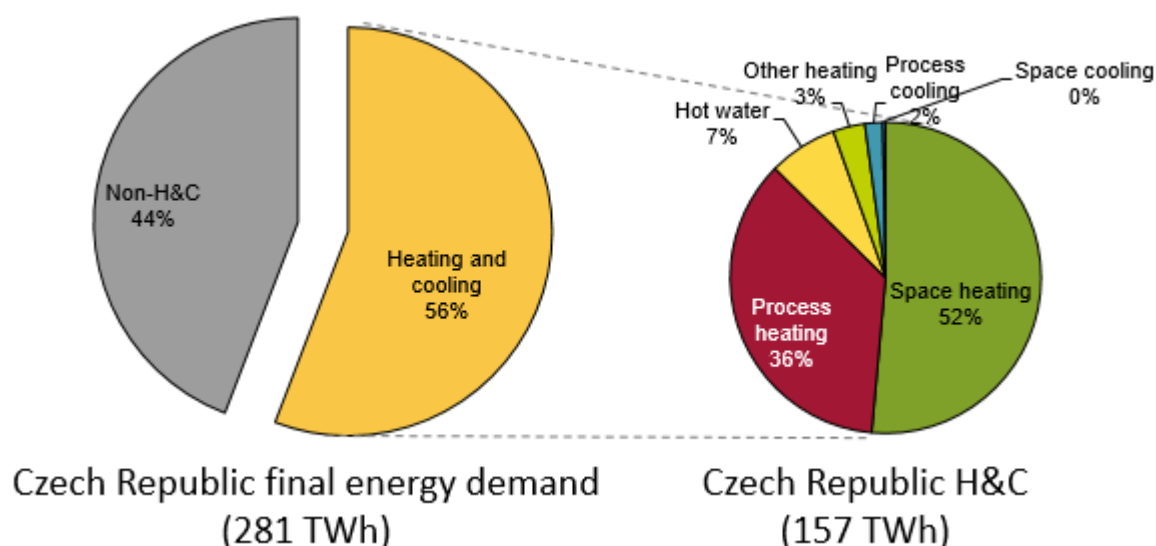
Figure 4. Heating and cooling demand in the Czech Republic by end-use compared to total final energy demand (2015 values).
