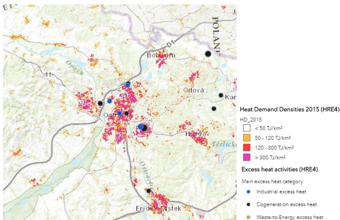
Figure 2. Heat demand density and excess heat activities Ostrava.
