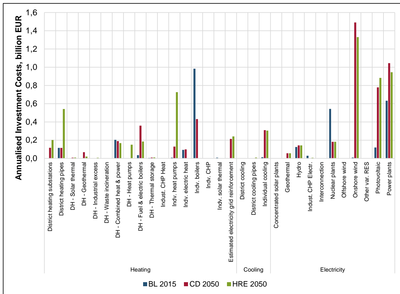
Figure 13. Annualised socio-economic investment costs and categories in the Czech Republic, excluding the investment costs necessary for energy savings.
