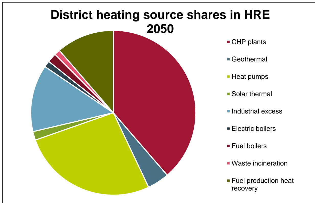
Figure 7. Heat sources for district heating in Heat Roadmap Czech Republic.
