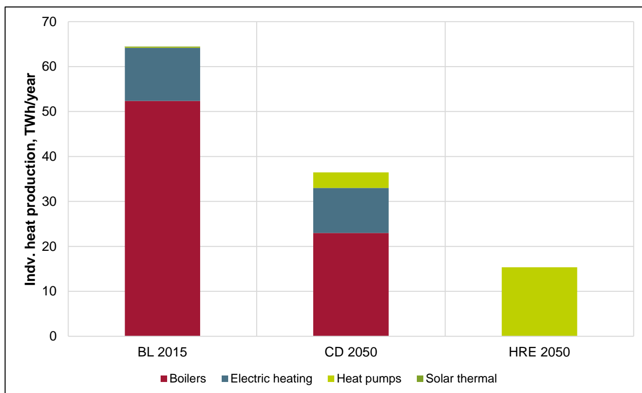
Figure 8. Heat sources for individual heat production in the Czech Republic for the three scenarios.
