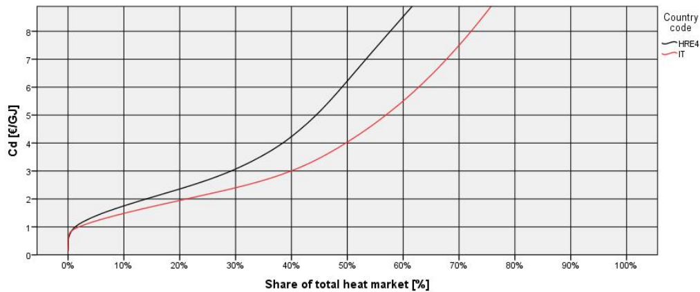
Figure 3. Distribution cost of heating at percentage share of total heat market for Italy and HRE average.
