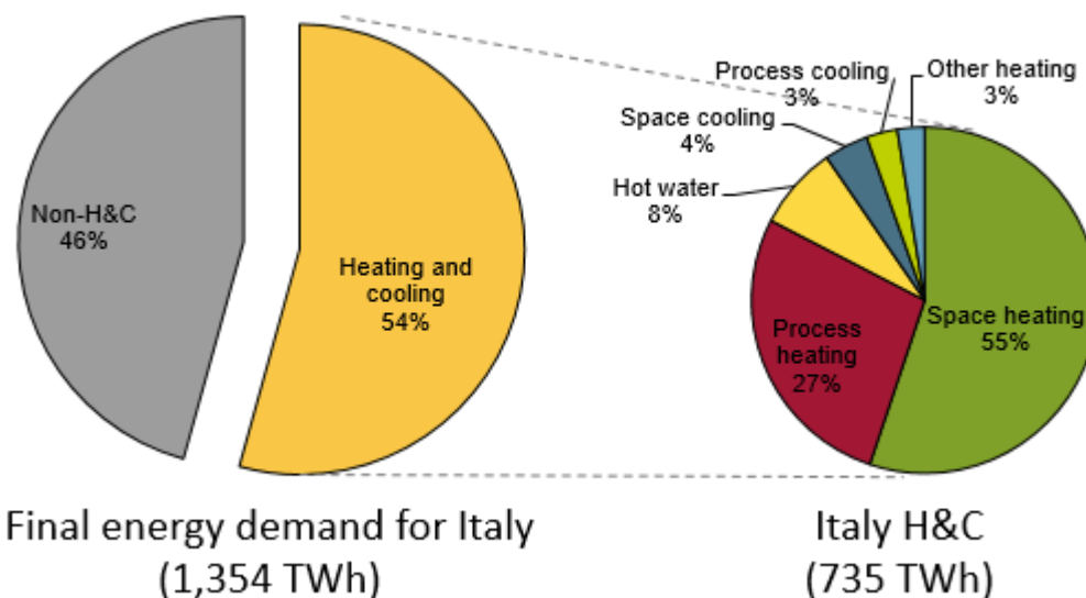
Figure 4. Heating and cooling demand in Italy by end-use compared to total final energy demand (2015 values).
