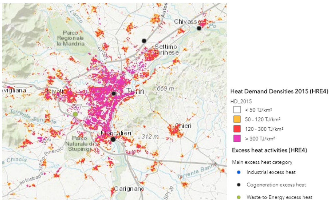
Figure 2. Heat demand density and excess heat activities Turin.
