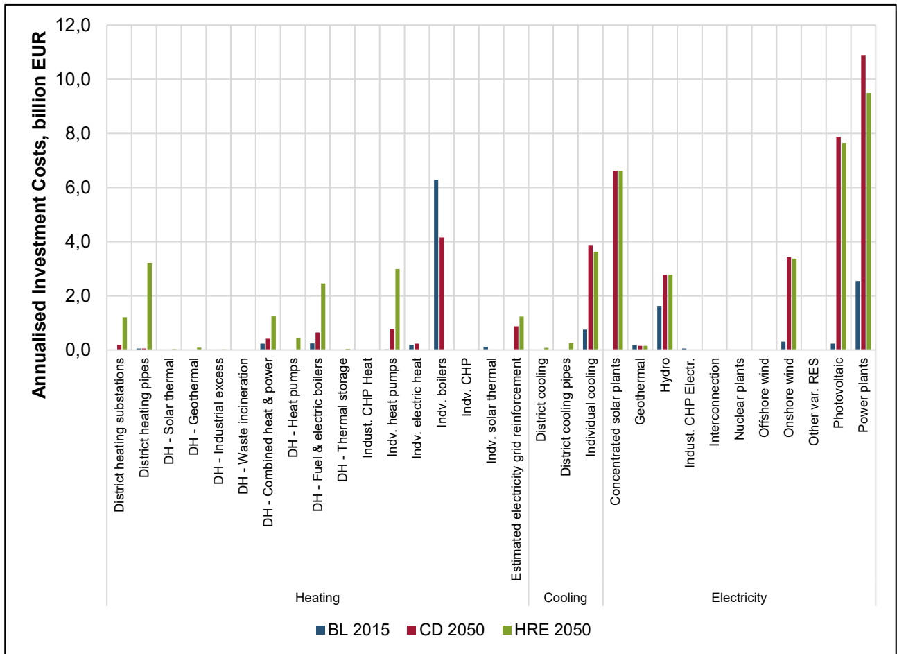
Figure 13. Annualised socio-economic investment costs and categories in Italy, excluding the investment costs necessary for energy savings.
