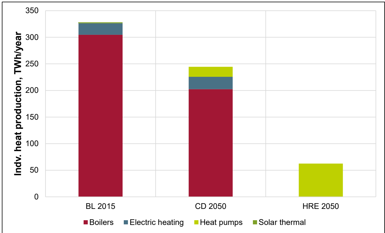
Figure 8. Heat sources for individual heat production in Italy for the three scenarios.
