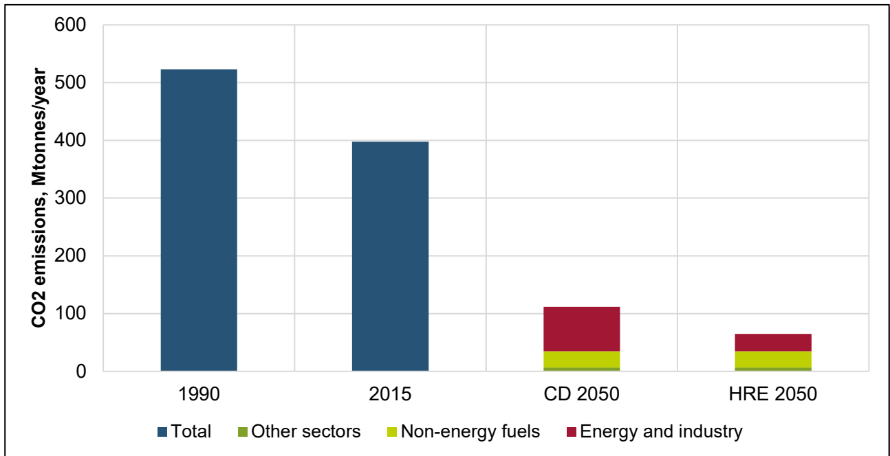
Figure 10. CO 2 emissions for Italy (including 1990, the base year for the Paris Agreement), currently, in a conventionally decarbonised scenario, and the Heat Roadmap scenario.
