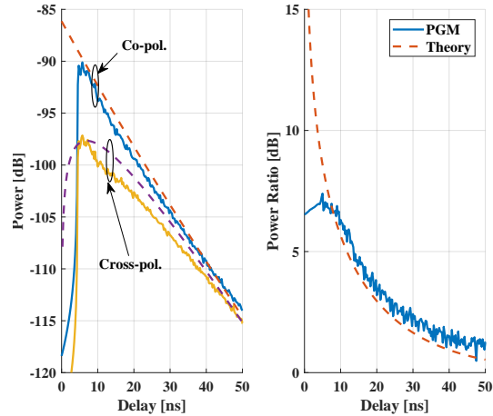
Fig. 3: Polarimetric power and power ratio from propagation graph and approximate expressions.
