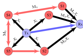
Fig. 1: PG for a polarized channel.
