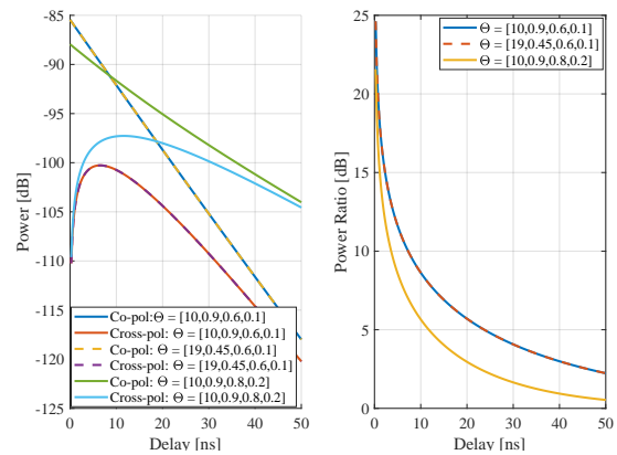
Fig. 4: Polarimetric power and power ratio with different parameters. \Theta denotes the parameter set [N_s, P_{\text{vis}}, g, \gamma] .
