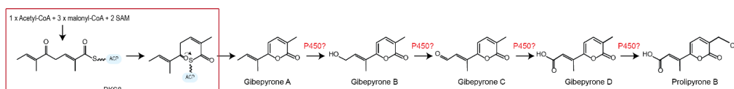
Figure 4. Proposed biosynthetic pathway of gibepyrone starting with production of gibepyrone A and ending with prolipyron B through oxygenation by one or several non-clustering cytochrome P450 monooxygenases.
