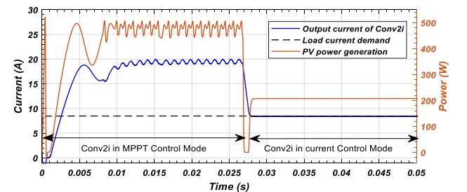
Fig. 7b. Power generated by PV panels in nanogrid 1 P_1^{PV} (right Y-axis) and output current I_1^m of conv2_i (left Y-axis) in case 5 (simulation results)
