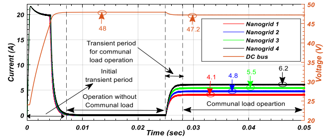
Fig. 3a. DC bus voltage V_B profile (right Y-axis) and current sharing among nanogrids ( I_1^L , I_2^L , I_3^L and I_4^L ) (left Y-axis) in case 1 (simulation results)
