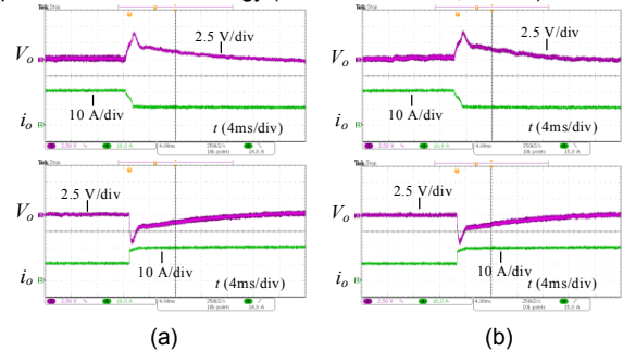
Fig. 14. Dynamic performances under load changes including V_o and i_o ( V_{in} = 550 V and V_o = 50 V). (a) Conventional asymmetrical modulation strategy. (b) Proposed modulation strategy.
