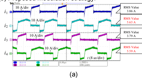
Fig. 8. Experimental results about currents i_1, i_2, i_3, and i_4 ( V_{in} = 550 \text{ V} , V_o = 50 \text{ V} , and P_o = 500 \text{ W} ). (a) Conventional asymmetrical modulation strategy. (b) Proposed modulation strategy.
