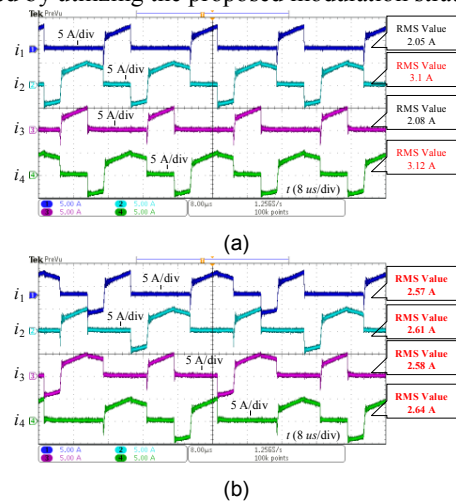
Fig. 8. Experimental results about currents i_1, i_2, i_3, and i_4 ( V_{in} = 550 \text{ V} , V_o = 50 \text{ V} , and P_o = 500 \text{ W} ). (a) Conventional asymmetrical modulation strategy. (b) Proposed modulation strategy.
