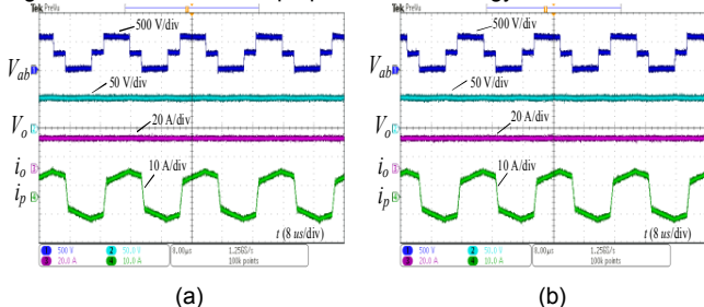
Fig. 7. Experimental results including V_{ab}, V_o, i_o, and i_p ( V_{in} = 550 \text{ V} , V_o = 50 \text{ V} , and P_o = 1 \text{ kW} ). (a) Conventional asymmetrical modulation strategy. (b) Proposed modulation strategy.
