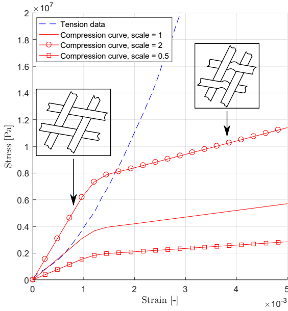
Figure 16. Scalable compression stress-strain curve with break caused by meso-level buckling.
