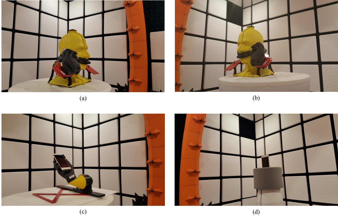
Fig. 1: Setup for: (a) voice service test with phone next to the right-hand side of the head phantom placed in the right hand phantom (beside head hand right - BHHR), (b) voice service test with phone next to the left-hand side of the head phantom placed in the left hand phantom (beside head hand left - BHHL), (c) data service test with phone placed in the right hand phantom (hand right - HR), and (d) voice and data service test with phone placed in free space (FS).
