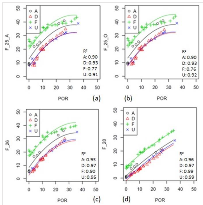
Figure 5-1 Best-fit models (with categorization) of the linear regression analyses of the POR index (x-%) with the static metrics (y-%; F_{25\_A} : 25°C threshold all day, F_{25\_O} : 25°C threshold occupied hours, F_{26} : 26°C threshold occupied hours, and F_{28} : 28°C threshold occupied hours) for all the variants (A: Austria, D: Denmark, F: South France, and U: U.K.; 31: p.7).
