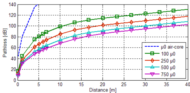
Figure 6.6: Pathloss versus distance between coils at 3000 Hz
