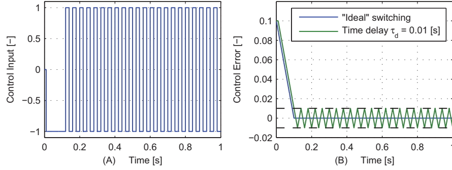
Figure 4.7: (A) Input of delayed relay control. Here, the ideal control is not depicted, as this is constituted by switching between \pm 1 with a frequency of 100 \text{ [kHz]} . (B) Control error of the system with and without delayed relay control. The dotted lines indicates the expected oscillation amplitude a_{ds} , resulting from the time delay \tau_d .
