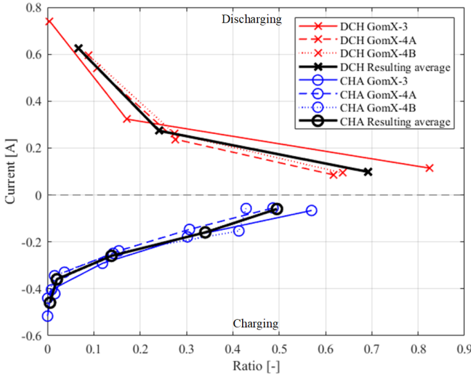
Fig. 3. Charging and discharging currents and their relative occurrence for GOMX nano-satellites and the resulting average values.
