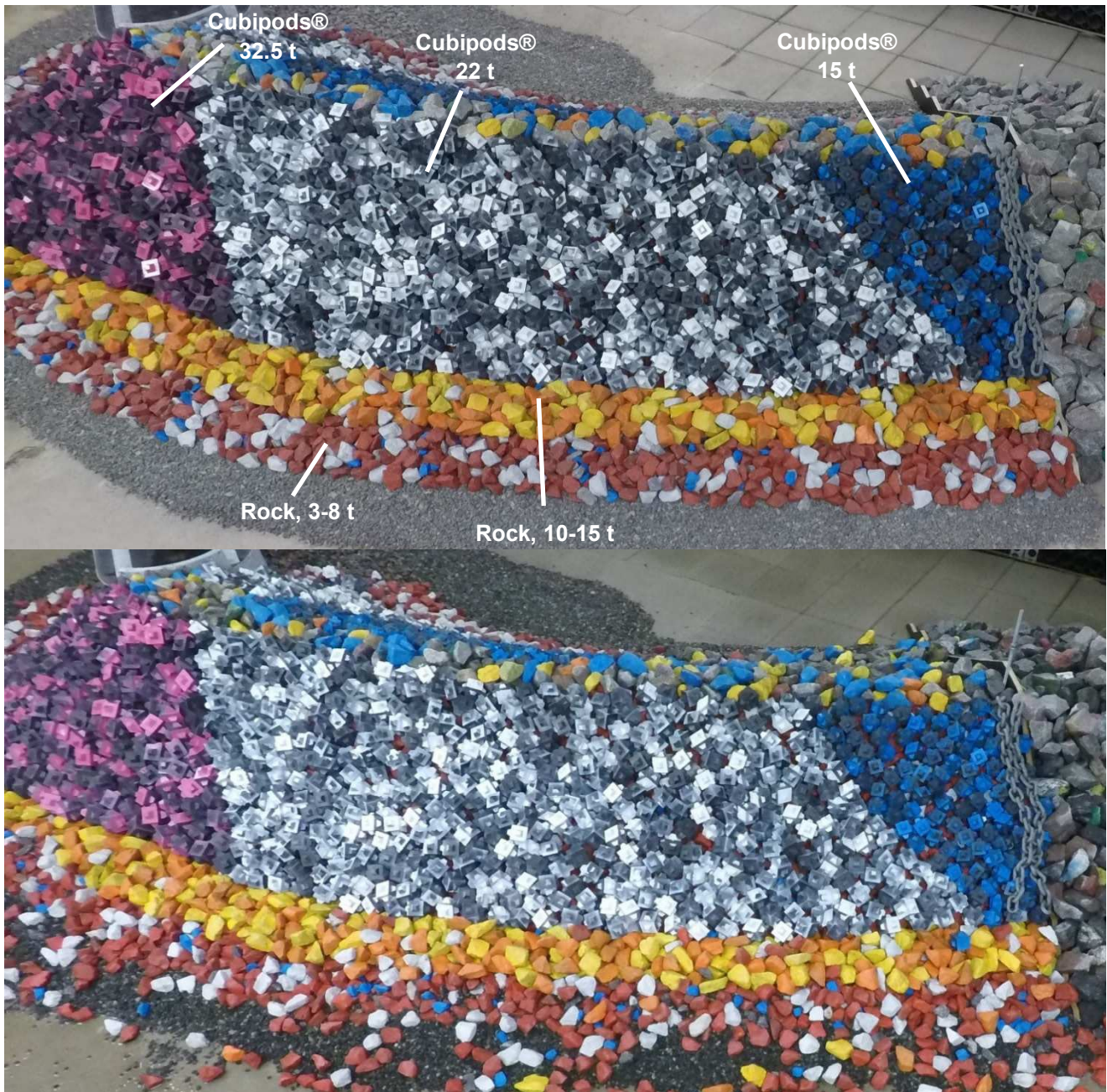
Fig. 6. Trunk section before testing (top) and after overload conditions (bottom).
