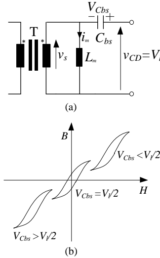
Fig. 10. Illustrations of (a) transformer equivalent circuit and (b) its B-H curves for demonstrating voltage stability of dc blocking capacitor.
