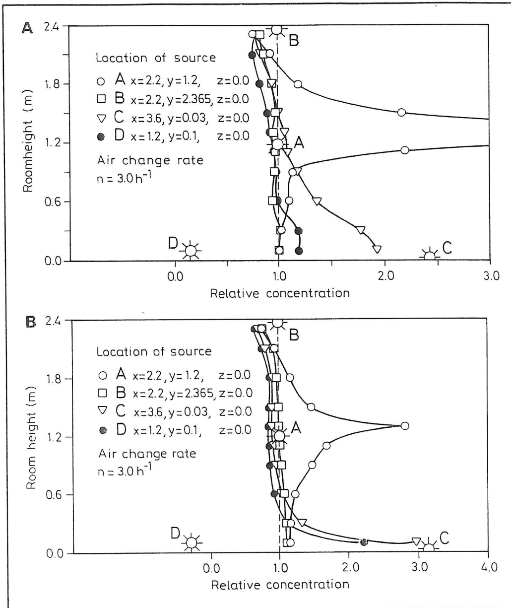
Figure 3. Relative concentration profiles for four different locations of the contamination source found by A) a passive tracer gas method and B) a conventional tracer gas method.
