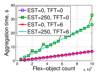
Fig. 13. Flex-offer aggregation time: for various FOs count
