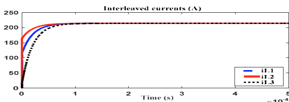
Fig.9. Inductor currents
