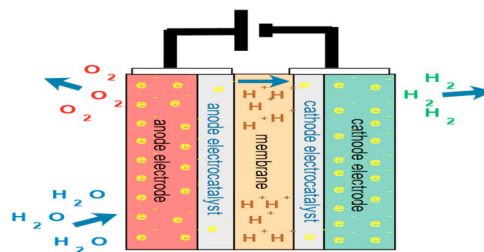
Fig.1: Presentative schema of PEM Electrolyzer cell
