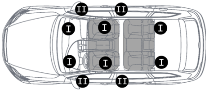
(a) Setup in a car cabin with the front seats being the bright zone and the rear seats the dark zone. Ten woofers were used in the experiment, six of type I and four of type II distributed as indicated.
