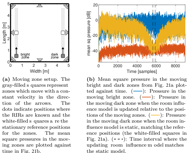
Fig. 21: Results and plots repeated from paper G [77]. Comparison of two zones moving with constant velocity along the trajectories indicated by the arrows and the control filters being updated along with the zone position or just being optimized for one fixed position.
