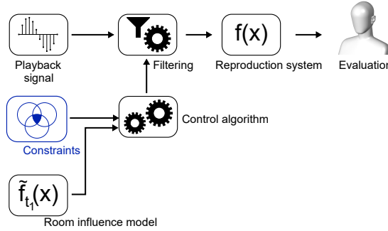
Fig. 18: Feed-forward control structure used for the investigation in paper C. The blue highlighted block indicate that the main focus is expressing the added constraint on pre- and post-ringing of the reproduced audio in the bright zone.
