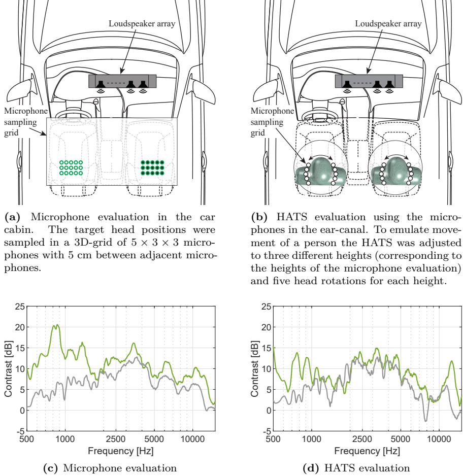
Fig. 17: Results and plots repeated from Paper F [76]. Contrast results attained with a planar loudspeaker array on the dashboard of a car, see Fig. 11c. The contrast is evaluated with the driver's seat as the bright zone and the front passenger seat as the dark zone. Delay and sum beamformer (—) and in situ control (—) in an automotive cabin, evaluated with microphones and with a HATS. Note that the contrast results have been smoothed with a 1/12^{\text{th}} -octave rectangular window to improve the readability of the results.
