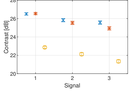
(b) Contrast. Note that these results are determined in the time-domain, hence, the contrast is the ratio of spatially averaged squared pressures in the bright and dark zone at each time sample. For detailed description see Paper G [77].
