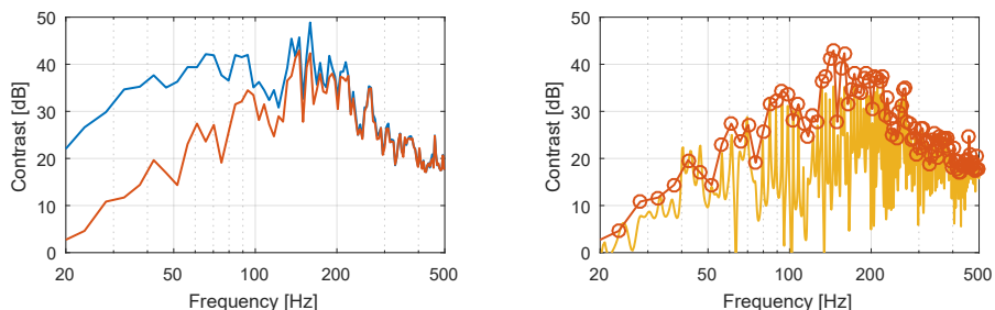
(a) Contrast results for two conditions: Loudspeaker control filters determined using room influence model 1 and evaluated using room influence model 1 (—). Loudspeaker control filters determined using room influence model 1 and evaluated using model 2, which is measured approximately 10 seconds after model 1 (—).
