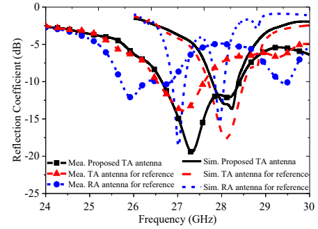
Fig. 18. Measured and simulated reflection coefficients of the RA antenna for reference, the proposed TA antenna, and the TA antenna for reference.
