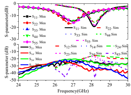
Fig. 19. Measured and simulated S-parameter of the beam-steerable TA antenna.
