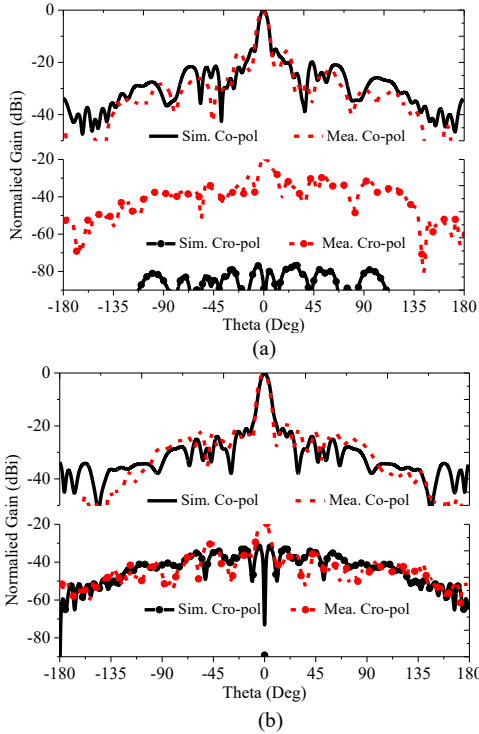
Fig. 21. Measured and simulated normalized radiation patterns of the proposed TA antenna. (a). E-plane. (b). H-plane (Due to the frequencies shifting for the measured results, the measured radiation patterns at 27.6 GHz and the simulated radiation patterns at 28.0 GHz are compared)
