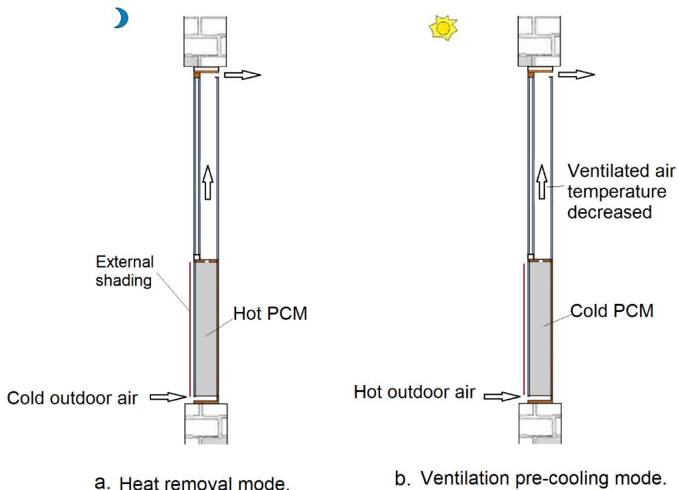
Fig. 3. Working principle of the PCMVW system in ventilation pre-cooling application.
