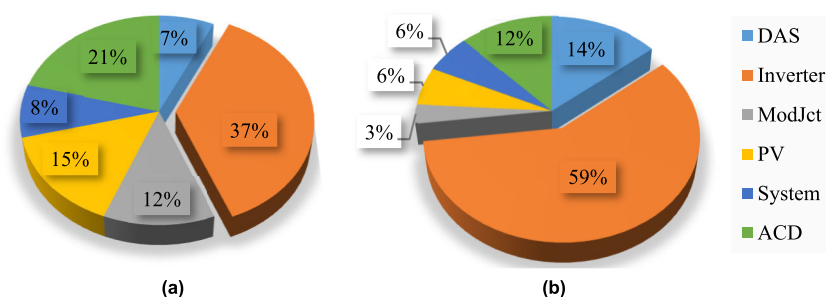
FIGURE 2. Five-year experience of failures in a commercial PV power plant in Arizona from 2001 to 2006 (DAS: Data Acquisition System, ACD: ac disconnects, ModJct: Module Junction Box, PV –PV arrays): (a) unscheduled maintenance events and (b) associated maintenance costs [11].
