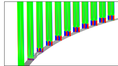
Figure 20. Vorticities for 0.8 mm 3D ZZ tape
