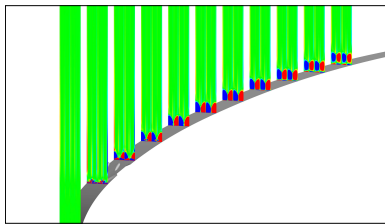
Figure 19. Vorticities for 0.6 mm 3D ZZ tape
