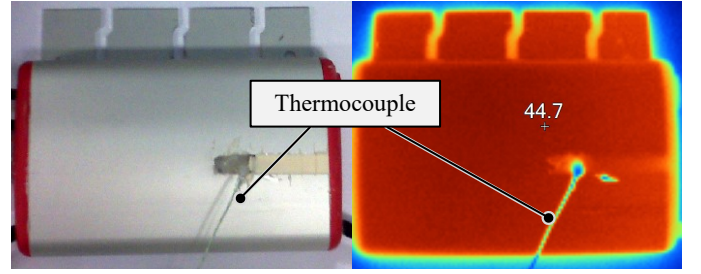
Fig. 8. Hardware prototype of the PV inverter: (a) picture of the prototype with integrated thermal sensor for the dc-link capacitor and (b) the thermal image acquired at the rated power and ambient temperature of 28°C.
