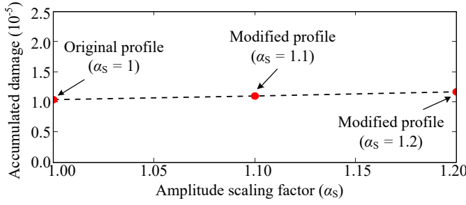
Fig. 16. Accumulated damage of capacitor under daily mission profile with different solar irradiance amplitude scaling factors (ambient temperature of T_a = 25^\circ\text{C} ).
