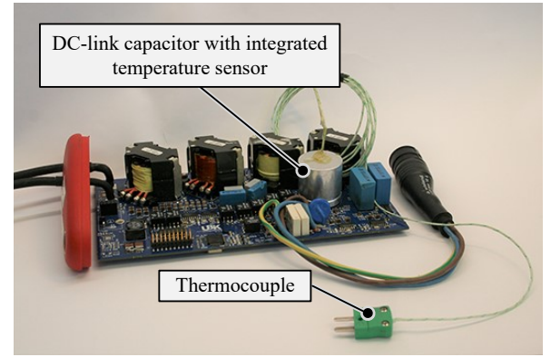
Fig. 2. Hardware prototype of the PV inverter where a thermocouple has been integrated with the dc-link capacitor.
