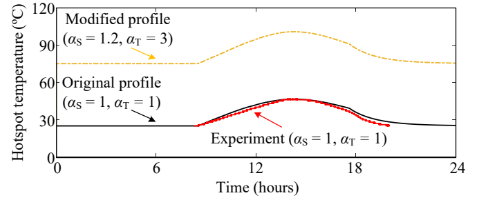
Fig. 19. Daily hotspot temperature of the dc-link capacitor with the amplitude scaling factors of \alpha_S = 1.2 and temperature scaling factors of \alpha_T = 3 .
