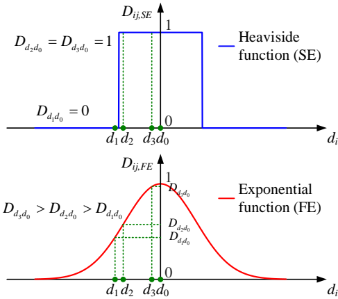
Fig. 3. The similarity function used to calculate SE and FE. The Heaviside function and the exponential function is for SE and FE calculation, respectively.
