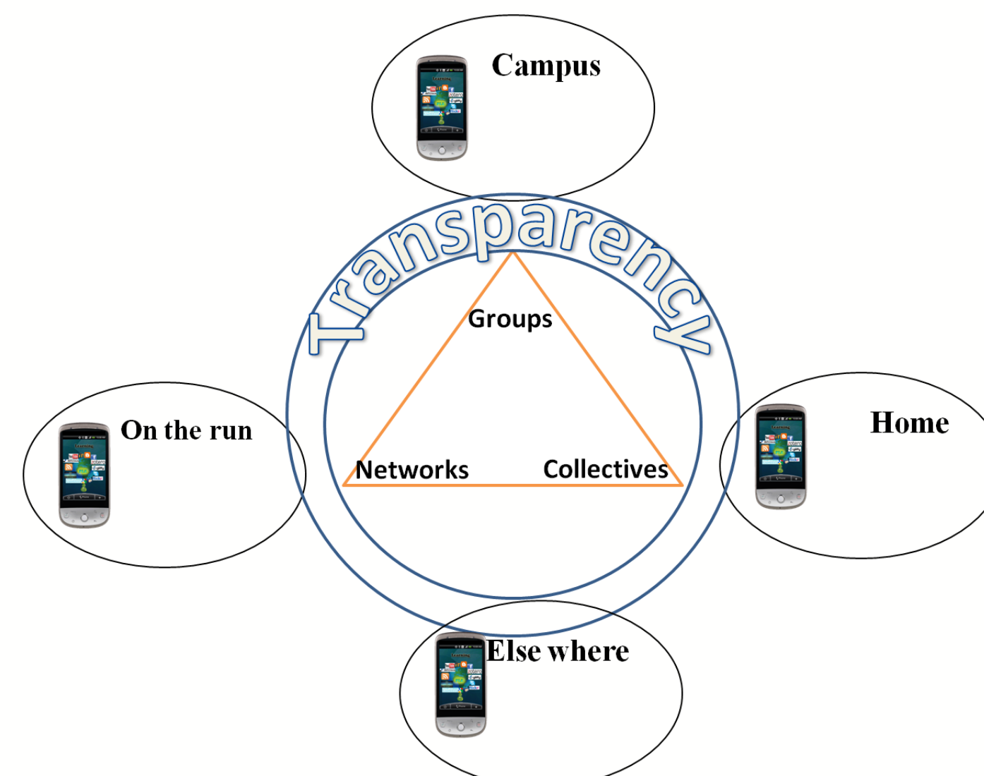
Figure5. Theoretical framework
