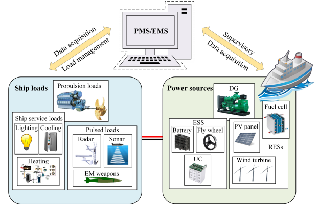
Fig. 1. Overall structure of PMS/EMS integrated SPS
