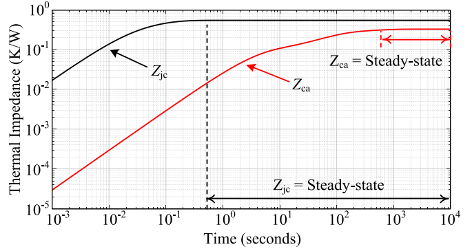
FIGURE 5. Thermal impedance of the IGBT module between junction and case Z_{jc} as well as case and ambient Z_{ca} [40].
