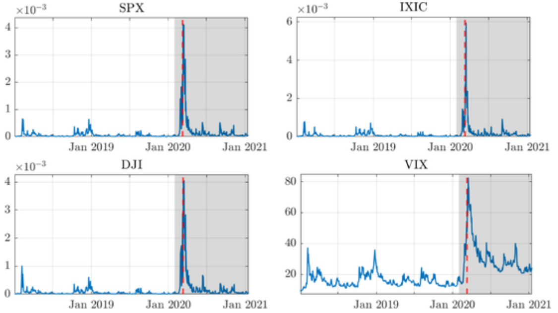
Fig. 1. Volatility indexes. The shaded area covers from the World Health Organization’s declaration of a Public Health Emergency of International Concern. The vertical red line signals the formal declaration of a pandemic.
