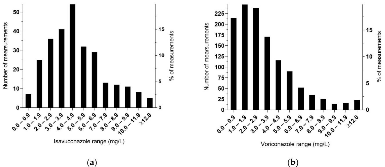
Figure 1. Distribution range of serum concentrations. (a) 273 s-ISZ concentrations measured from 35 patients at SSI. Patients received various dosages and the plots do not describe exposures after administration of standard dosing. (b) 1242 s-VRZ concentrations measured from 283 patients.
