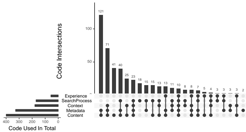
Figure 4: Visualization of the co-occurrence between top-level relevance aspect categories in known-item requests. Vertical bars represent how often the combinations of top-level aspects co-occurred in our sample ( N = 462 ).
