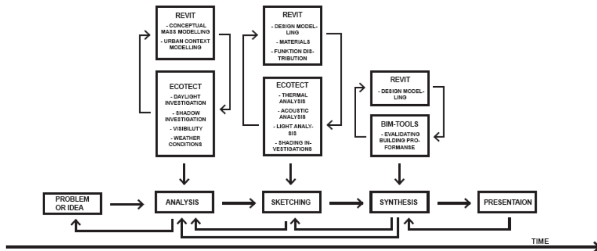
Figure 2. The phases in the integrated design process where Revit and Ecotect can be implemented.
