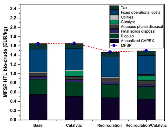
Figure 6. Effect of \text{K}_2\text{CO}_3 addition and aqueous phase recirculation on the final MFSP.
