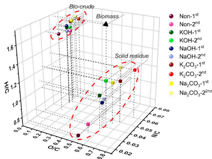
Figure 4. Van Krevelen 3D scatter plot of bio-crude, solid residue, and biomass samples.
