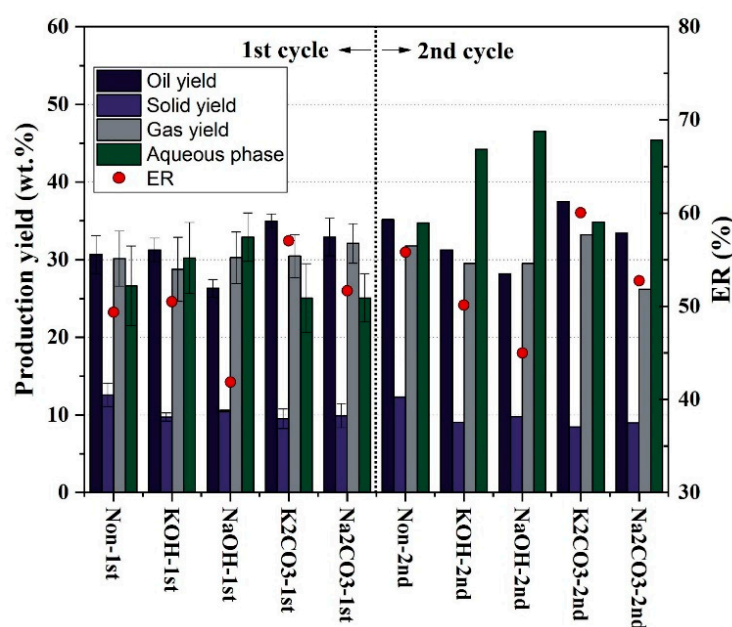
Figure 1. Distribution of HTL products and ER of bio-crude.
