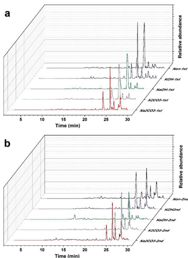
Figure 5. GC-MS analysis results of (a) first cycle- and (b) second cycle-driven bio-crudes.
