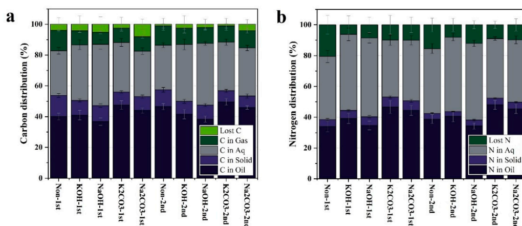
Figure 3. (a) Carbon and (b) nitrogen distribution among different HTL products.
