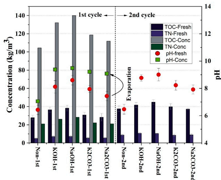
Figure 2. TOC, TN, and pH values of the fresh and concentrated aqueous phase.
