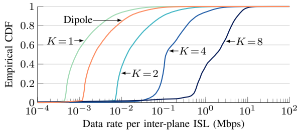
Fig. 2. CDF of the selected data rates per ISL with Butler matrix having K = \{1, 2, 4, 8\} antenna ports and a half-wave dipole antenna for \Delta t = 30 s.
