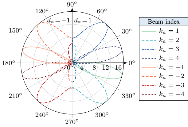
Fig. 1. Antenna gains per beam along the azimuth plane with two 4 \times 4 Butler matrix arrays with d_e = c/2f .
