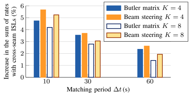
Fig. 3. Sum rate increase due to enabling cross-seam ISLs for the Butler matrix and digital beam steering with K = \{4, 8\} and for \Delta t = \{10, 30, 60\} .
