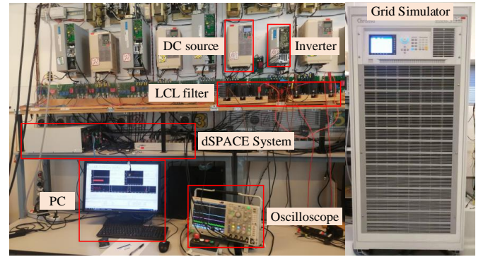
Fig. 18. Experimental setup.
