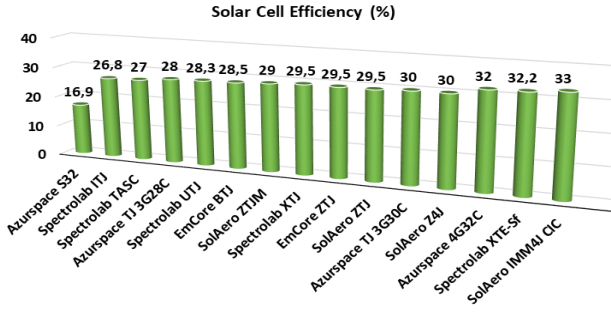
Fig. 20. Space solar cell technologies and their efficiencies [91], [92].
