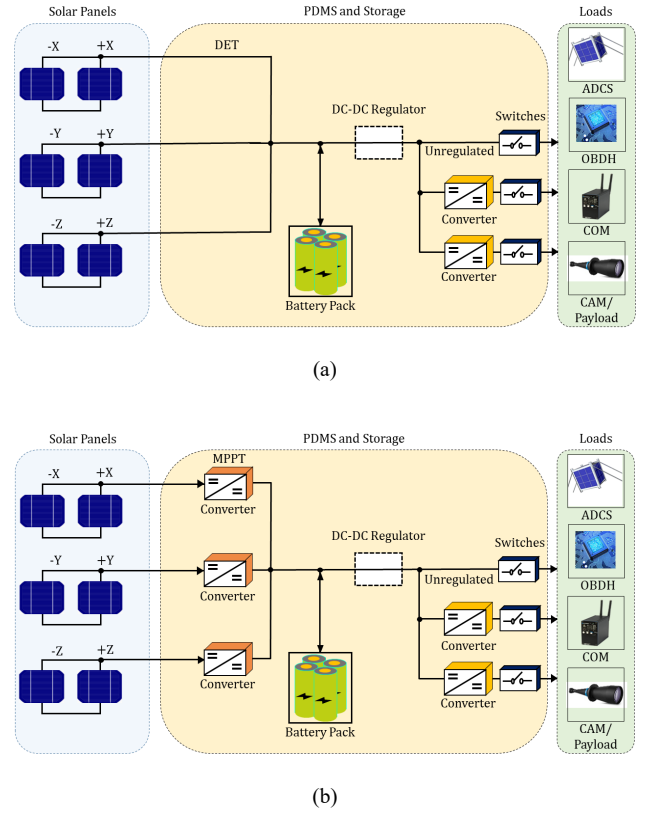
Fig. 2. The two basic architectures of EPS (a) DET solar power conversion and (b) MPPT solar power conversion topologies with unregulated buses.
