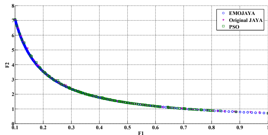
Figure 4. Comparison of the Pareto front from EMOJAYA, JAYA and PSO (Test Function 3).
