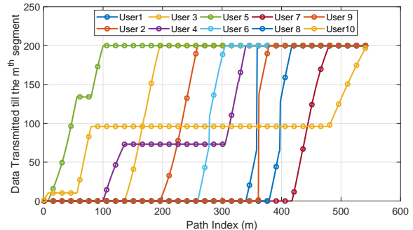
(b) Scheduling
