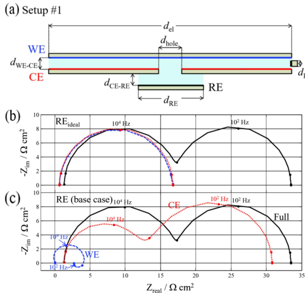
Figure 6. (a) Setup #1 with a hole in the CE of a three-electrode coin cell setup. Spectra are measured vs. (b) RE_{ideal} and (c) RE. [57]. Reprint with permission [57]; Copyright 2014, IOP Science.
